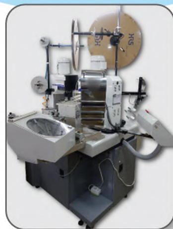
全自動防水密封插入高性能壓著機 Fully automatic waterproof single end seal
